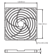
6G-120P for 120mm fan
